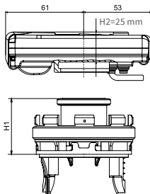
Combi version type ASF A1
