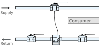
Asymmetrical sensor installation for zelsius® C5-CMF with one temperature sensor integrated in the flow sensor
