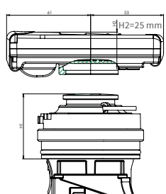
Combi version type A1
