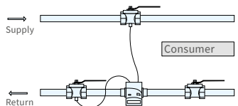
Symmetrical sensor installation for zelsius® C5-CMF
