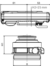
Combi version type IST, TE1, M60, PCC
